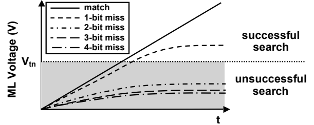
Fig. 6. Waveform of five matchline cases versus time in the error-correcting match scheme.
